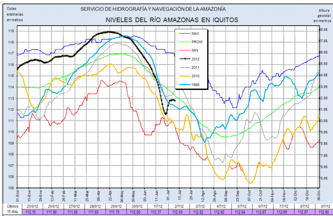
Amazon River levels in Iquitos: the blue line indicates historical maximum level of river, the green line average level, and the black line the level reached in 2012.
